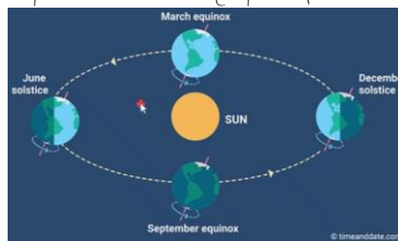
Seasons of the year according to heliocentrism.
